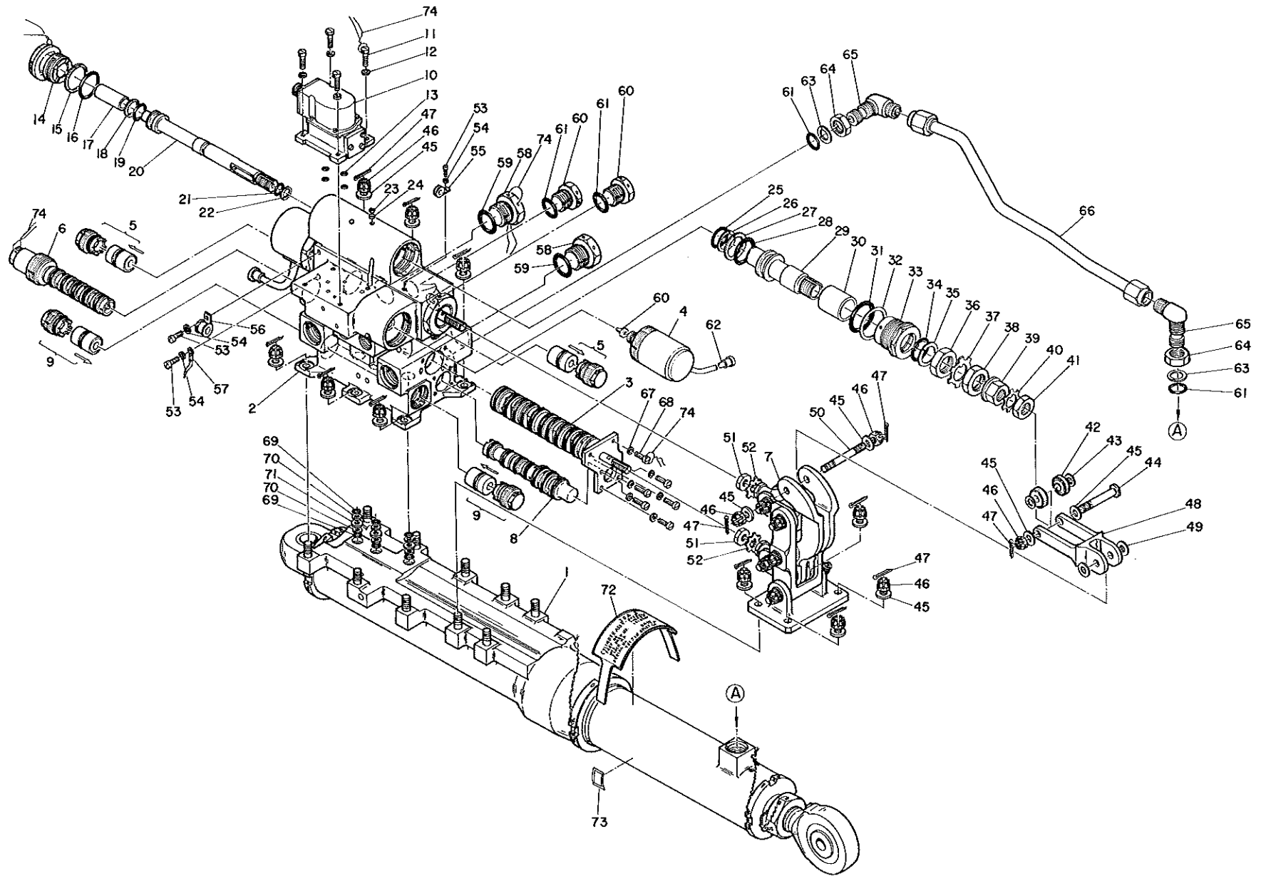
outboard Flap Servo Assembly
