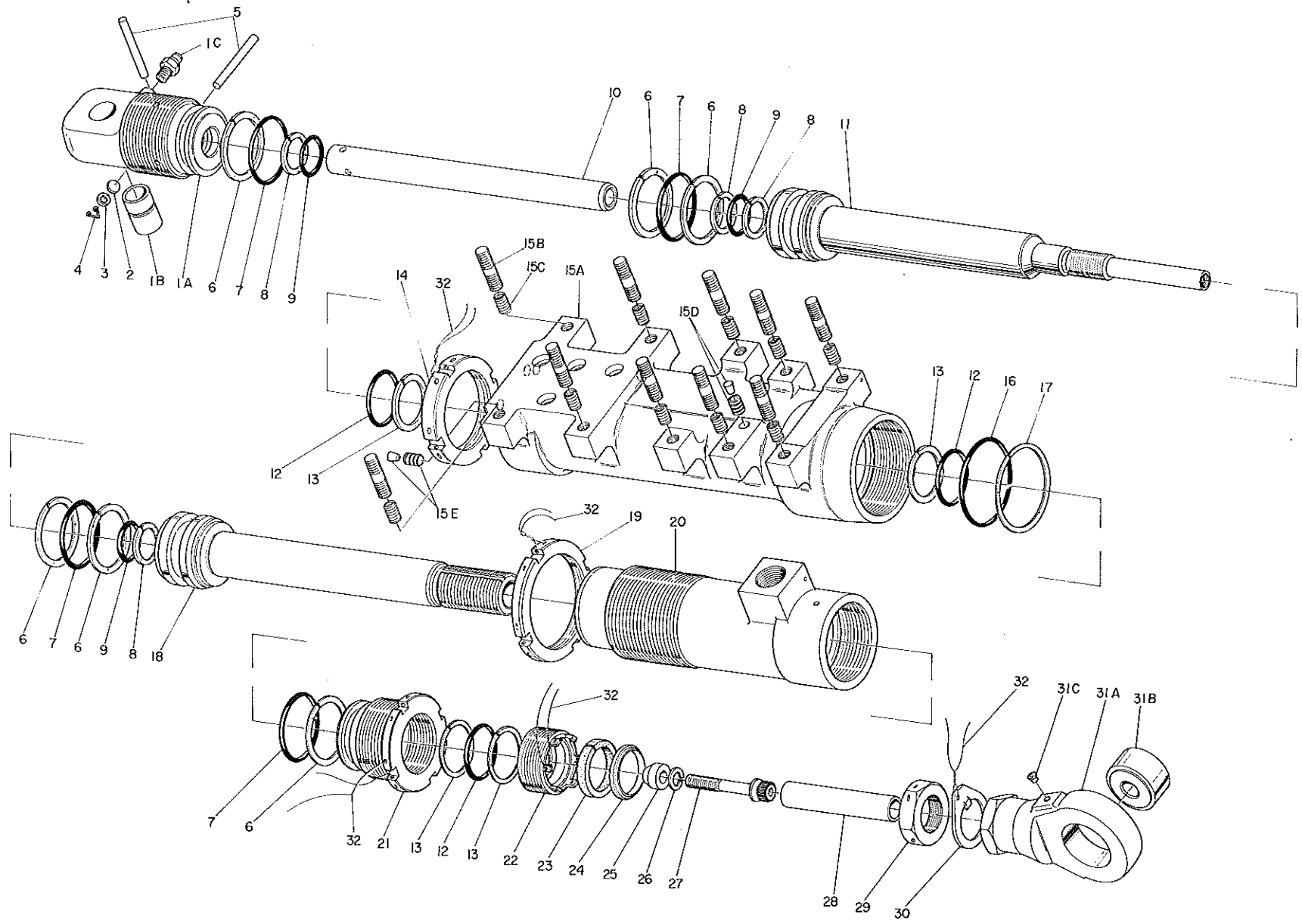
Cylinder Assembly Figure 102
