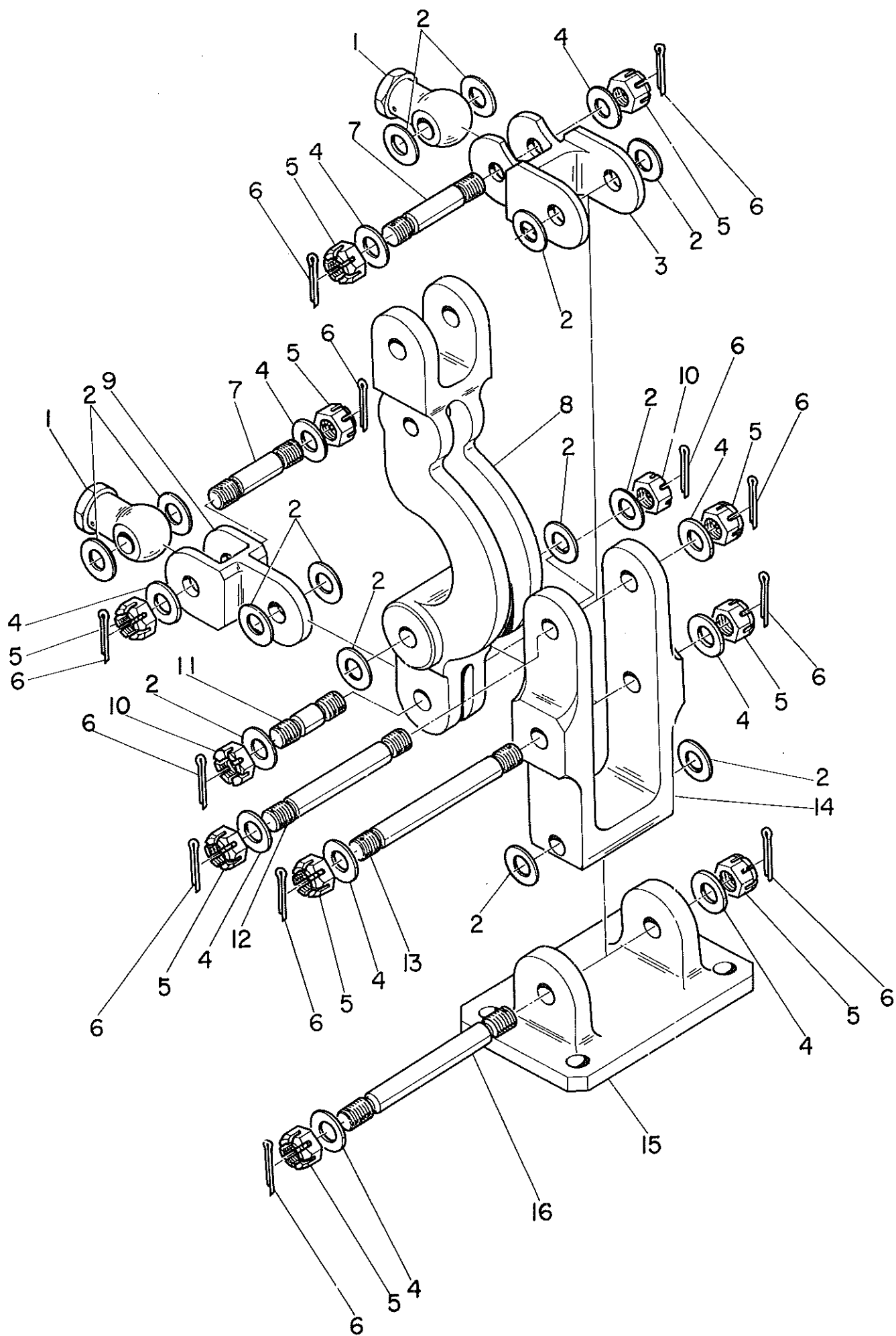
LINK ASSY
