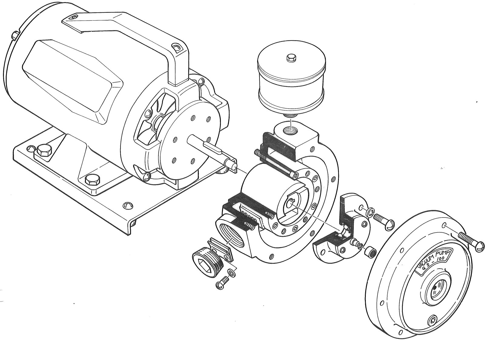
GS - 100 VACUUM PUMP
